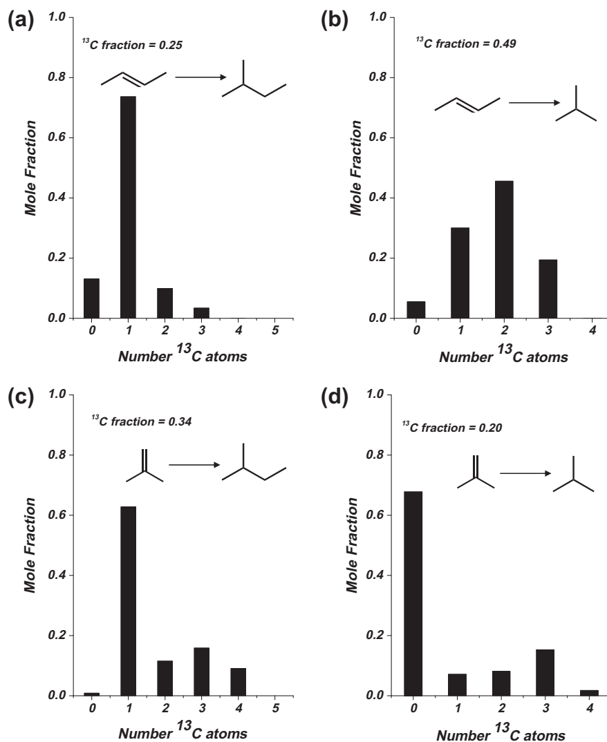
Fig. 3. Isotopologue distributions and ^{13}\text{C} -atomic fractions for (a) isopentane and (b) isobutane molecules produced from co-reaction of ^{13}\text{C} -labeled dimethyl ether (78 kPa) with ^{12}\text{C} -linear butene (0.5 kPa) and (c) isopentane and (d) isobutane molecules produced from co-reaction of ^{13}\text{C} -labeled dimethyl ether (78 kPa) with ^{12}\text{C} -isobutene (0.5 kPa). Reactions conducted at 473 K on H-BEA (Si/Al = 12.5) at space velocity of 0.025 mol inlet gas [mol Al s] ^{-1} with >90% alkene conversion and less than 5% total carbon conversion (DME and alkene).
