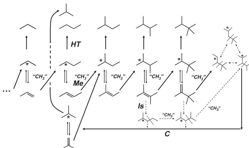
Scheme 2. Chain growth sequence for dimethyl ether homologation (starting with propene for simplicity). The asterisk indicates the position of alkoxide attachment to the surface. HT, Me, Is, and C labels represent hydrogen transfer, methylation, isomerization, and cracking reactions, respectively. “CH 3 ” represents surface methylating species derived from dimethyl ether.
