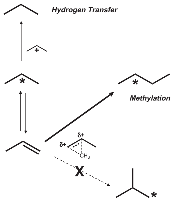
Scheme 3. Reaction pathways for C_3 species (propene and propoxide) in acid-catalyzed dimethyl ether homologation pathways. Methylation of propene occurs faster than hydrogen transfer to propoxide. Methylation of propene to isobutane does not occur because of the formation of a primary carbenium ion.
