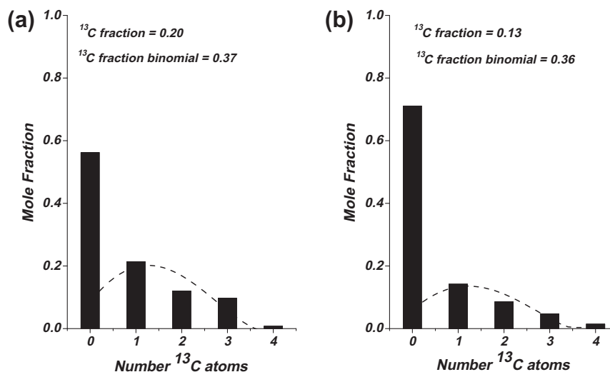
Fig. 8. Isotopologue distributions of (a) isobutane and (b) linear C_4 species produced from reactions between ^{13}C -labeled dimethyl ether (78 kPa) and ^{12}C -3,4,4-trimethyl-2-pentene (0.5 kPa) at 473 K on H-BEA (Si/Al = 12.5). Reactions conducted at 473 K and space velocity of 0.025 mol inlet gas [mol Al s] ^{-1} with >90% alkene conversion and less than 5% total carbon conversion (DME and alkene).
