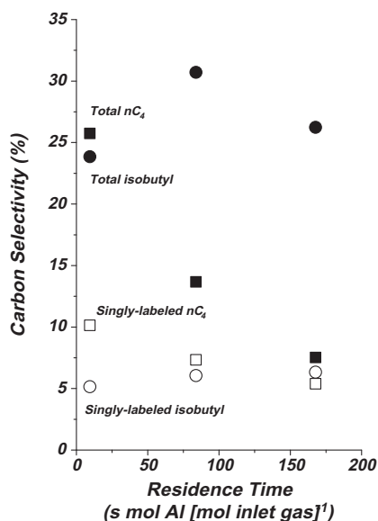
Fig. 1. Selectivity (% carbon basis) to linear C 4 species and isobutyl species as a function of reactor residence time (s mol Al [mol inlet gas] -1 ) for reactions between 13 C-labeled dimethyl ether (84 kPa) and unlabeled propene (2 kPa) at 473 K on H-BEA (Si/Al = 12.5). Total carbon conversions were less than 5%.
