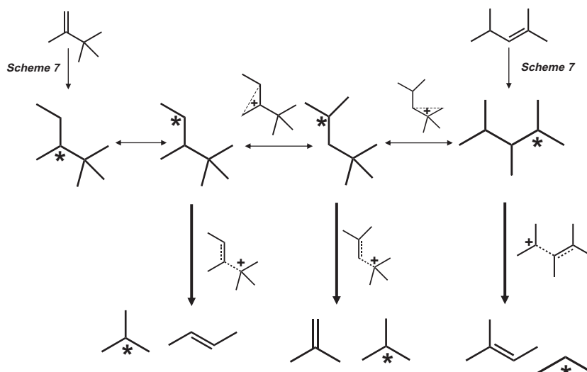
Scheme 8. \beta -Scission pathways for trimethylpentoxides that form from methylation of triptene and 2,4-dimethyl-2-pentene. \beta -Scission of 3,4,4-trimethyl sec -pentoxide and 2,4,4-trimethyl sec -pentoxide occurs more rapid than \beta -scission of 2,3,4-trimethyl sec -pentoxide.
