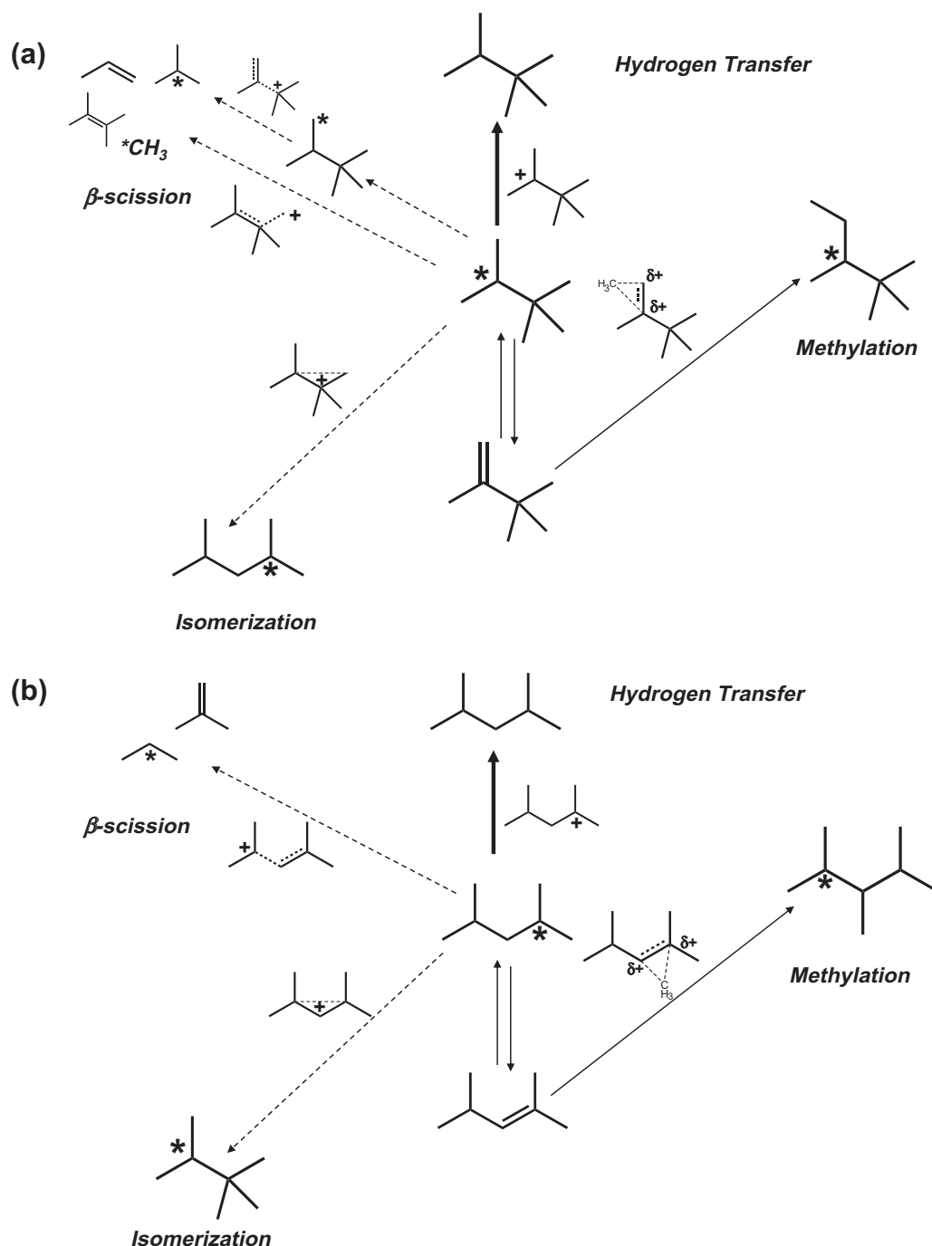
Scheme 7. Reaction pathways for (a) triptyl species (triptene and 2,3,3-trimethyl sec -butoxide) and (b) dimethyl-pentyl species (dimethyl-pentenes and 2,4-dimethyl sec -pentoxide) in acid-catalyzed dimethyl ether homologation pathways. Methylation of triptene to 3,4,4-trimethyl sec -pentoxide occurs much more slowly than hydrogen transfer to 2,3,3-trimethyl sec -butoxide. Methylation of methyl-pentenes to 2,3,4-trimethyl sec -pentoxide occurs faster than hydrogen transfer to 2,4-dimethyl sec -pentoxide. Isomerization and \beta -scission of both 2,3,3-trimethyl sec -butoxide and 2,4-dimethyl sec -pentoxide occur much more slowly than hydrogen transfer to these alkoxydes and methylation of their alkenes.
