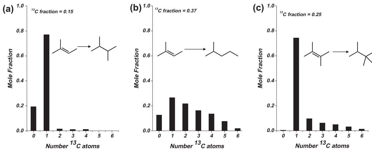
Fig. 4. Isotopologue distributions and ^{13}\text{C} -atomic fractions of (a) 2,3-dimethylbutane molecules and (b) 2-methylpentane molecules produced from co-reaction of ^{13}\text{C} -labeled dimethyl ether (78 kPa) with ^{12}\text{C} -2-methyl-2-butene (0.5 kPa) and (c) triptane molecules produced from co-reaction of ^{13}\text{C} -labeled dimethyl ether (78 kPa) with ^{12}\text{C} -2,3-dimethyl-2-butene (0.5 kPa). We use the 85 amu fragment of triptane as a surrogate for the parent ion, because the former appears in much higher concentrations in the mass spectrometer than the latter. Reactions conducted at 473 K on H-BEA ( \text{Si}/\text{Al} = 12.5 ) at space velocity of 0.025 mol inlet gas [\text{mol Al s}]^{-1} with >90% alkene conversion and less than 5% total carbon conversion (DME and alkene).
