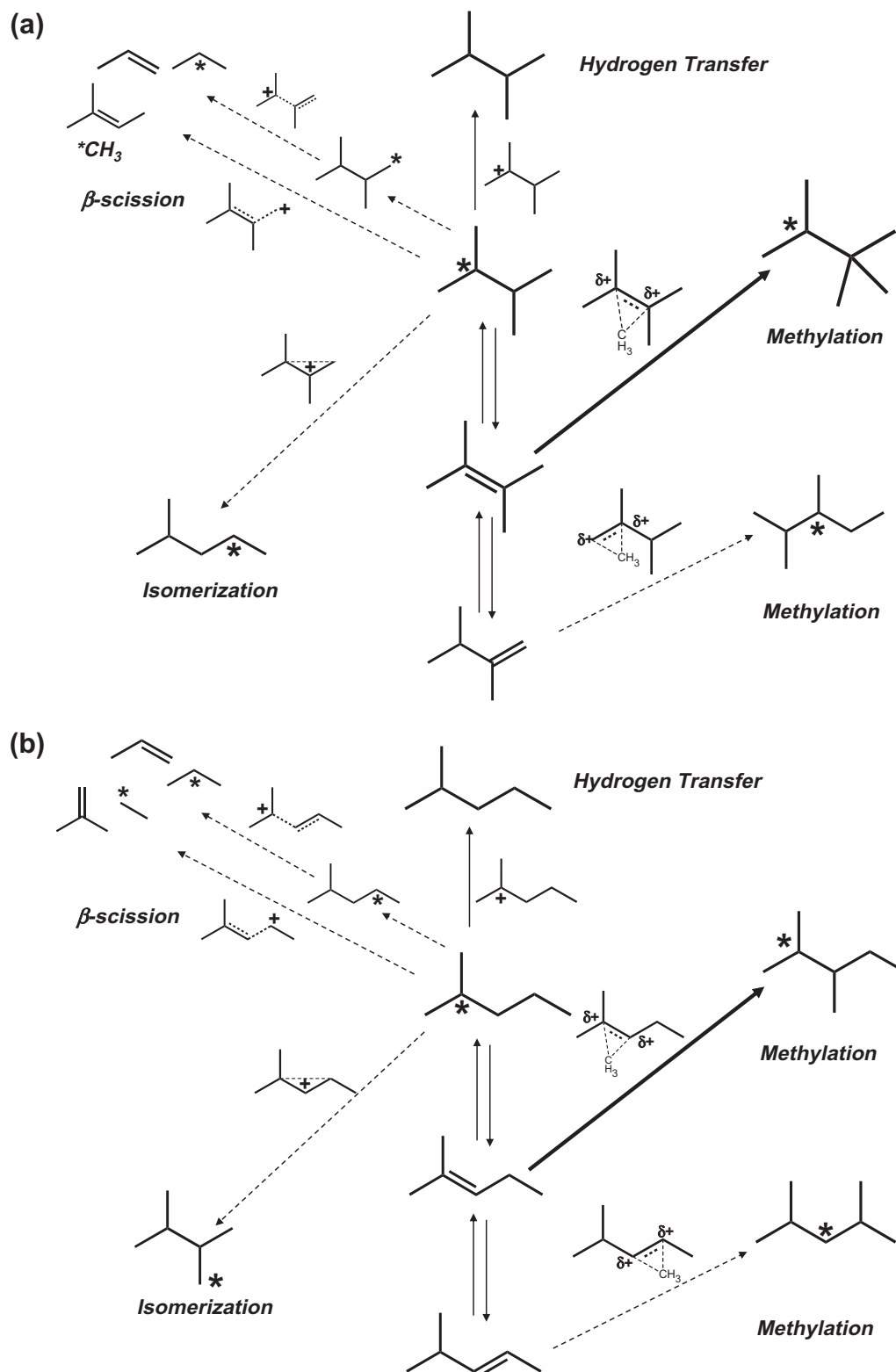
Scheme 6. Reaction pathways for (a) 2,3-dimethylbutyl species (2,3-dimethylbutenes and 2,3-dimethyl sec -butoxide) and (b) methyl-pentyl species (methyl-pentenes and 2-methyl sec -pentoxide) in acid-catalyzed dimethyl ether homologation pathways. Methylation of 2,3-dimethylbutenes to triptyl species occurs faster than hydrogen transfer to 2,3-dimethyl sec -butoxide. Methylation of methyl-pentenes to dimethyl-pentyl species occurs faster than hydrogen transfer to 2-methyl sec -pentoxide. Isomerization and \beta -scission of both 2,3-dimethyl sec -butoxide and 2-methyl sec -pentoxide occur much more slowly than hydrogen transfer to these alkoxides and methylation of their alkenes.
