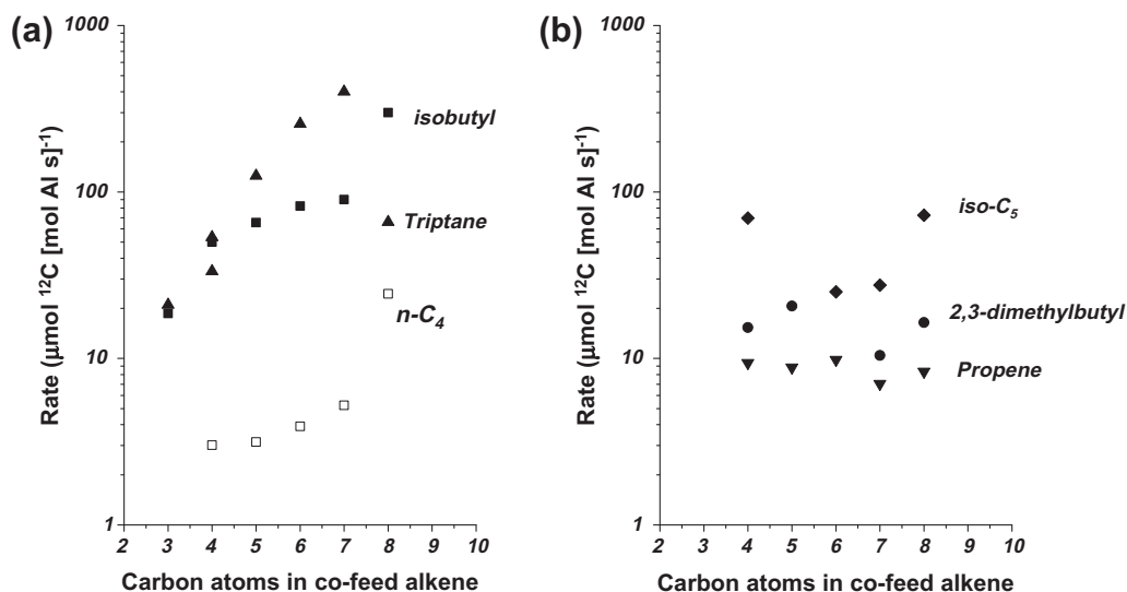
Fig. 6. Rate of formation ( ^{12}C -atomic basis) of (a) triptane (▲), isobutyl (■), and linear C_4 (□) species and (b) propene (▼), iso - C_5 (◆), and 2,3-dimethylbutyl (●) species for reactions between ^{13}C -labeled dimethyl ether (78 kPa) and 0.5 kPa unlabeled propene, trans -2-butene, 2-methyl-2-butene, 2,3-dimethyl-2-butene, triptene, or 3,4,4-trimethyl-2-pentene at 473 K on H-BEA (Si/Al = 12.5). Reactions conducted at 473 K and space velocity of 0.025 mol inlet gas [mol Al s] ^{-1} with >90% alkene conversion and less than 5% total carbon conversion (DME and alkene).
