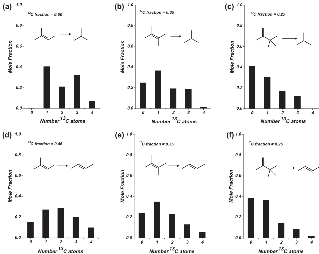
Fig. 5. Isotopologue distributions and 13 C-atomic fractions of isobutane (a–c) and trans-2-butene (d–f) molecules produced from co-reaction of 13 C-labeled dimethyl ether (78 kPa) with 0.5 kPa of 12 C-2-methyl-2-butene (panels a and d), 12 C-2,3-dimethyl-2-butene (panels b and e), and 12 C-triptene (panels c and f). Reactions conducted at 473 K on H-BEA (Si/Al = 12.5) and at a space velocity of 0.025 mol inlet gas [mol Al s] −1 with >90% alkene conversion and less than 5% total carbon conversion (DME and alkene).
