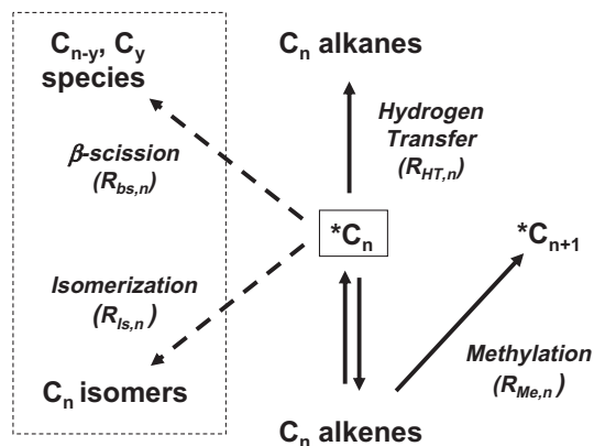
Scheme 1. Reaction pathways for alkenes and alkoxides formed as intermediates along dimethyl ether homologation pathways. Reactions denoted with solid lines occur faster than those denoted with dashed lines.
