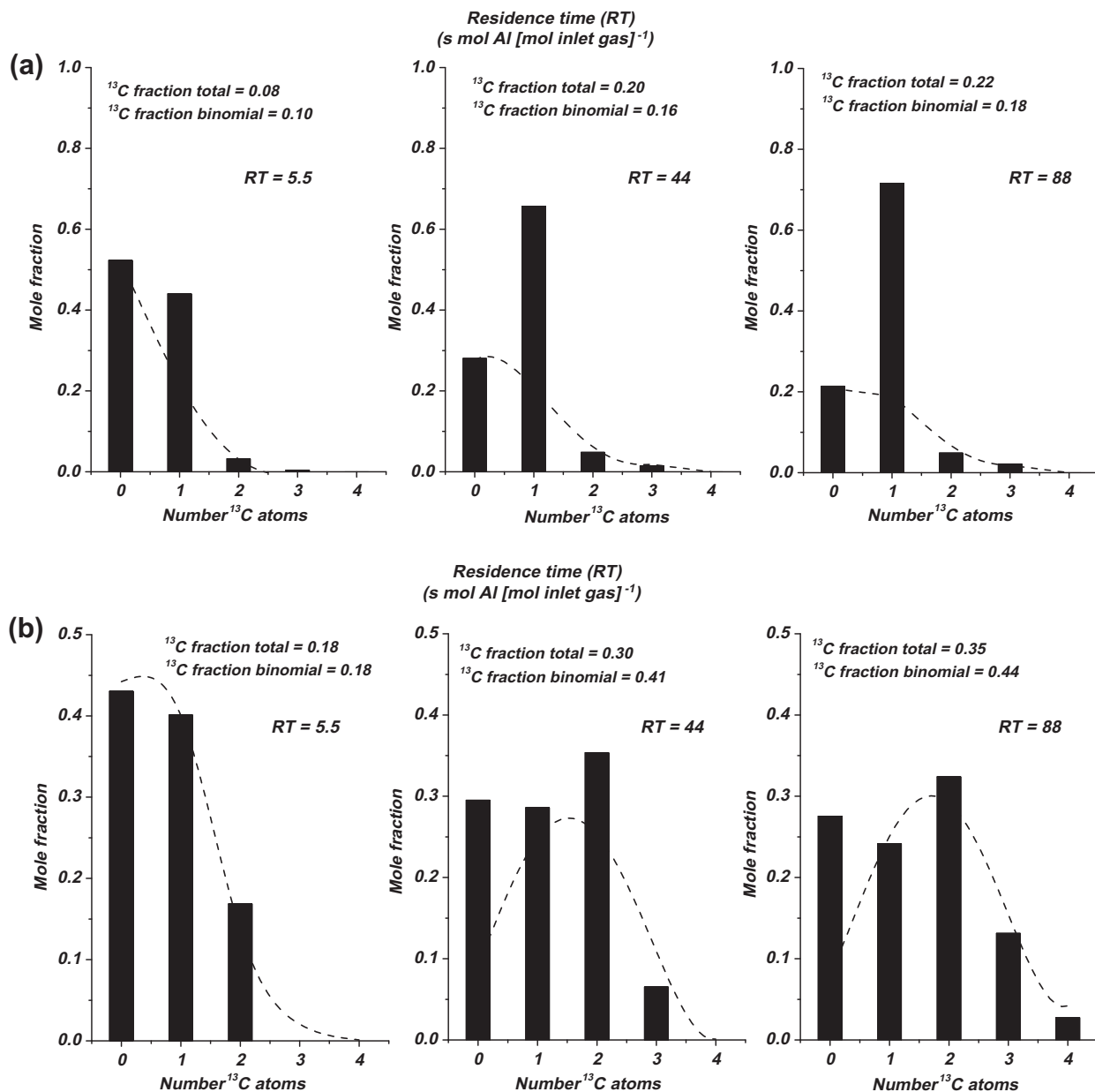
Fig. 2. Isotopologue distributions and ^{13}\text{C} -atomic fractions of (a) trans-2-butene and (b) isobutane molecules produced from reactions between ^{13}\text{C} -labeled dimethyl ether (84 kPa) and ^{12}\text{C} -propene (2 kPa) at 473 K on H-BEA at residence times of 5.5 (left), 44 (middle), and 88 (right) s mol Al [mol inlet gas] ^{-1} and propene conversions of 13% (left), 63% (middle), and 73% (right). Total carbon conversions (DME and propene) were less than 5%. The dashed markers indicate the binomial distribution expected for the ^{13}\text{C} -fraction in the binomial portion present in each particular chemical species [8].
