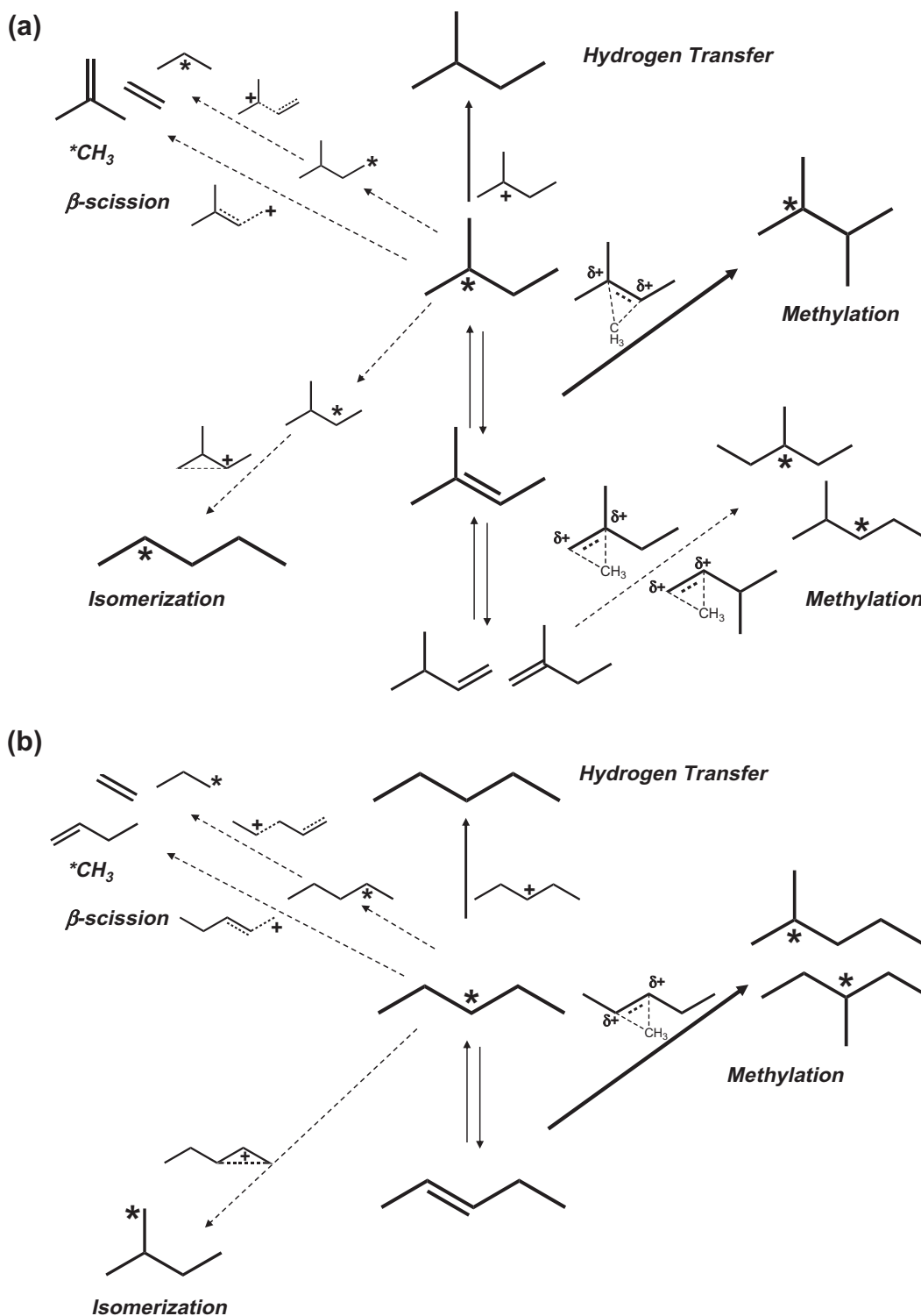
Scheme 5. Reaction pathways for (a) isopentyl species (isopentenes and 2-methyl sec -butoxide) and (b) n -pentyl species ( n -pentenes and sec -pentoxide) in acid-catalyzed dimethyl ether homologation pathways. Methylation of isopentene to 2,3-dimethylbutyl species occurs faster than hydrogen transfer to 2-methyl sec -butoxide. Methylation of n -pentenes to methyl-pentyl species occurs faster than hydrogen transfer to sec -pentoxide. Isomerization and β-scission of both sec -pentoxide and 2-methyl sec -butoxide occur much more slowly than hydrogen transfer to these alkoxides and methylation of their alkenes.
