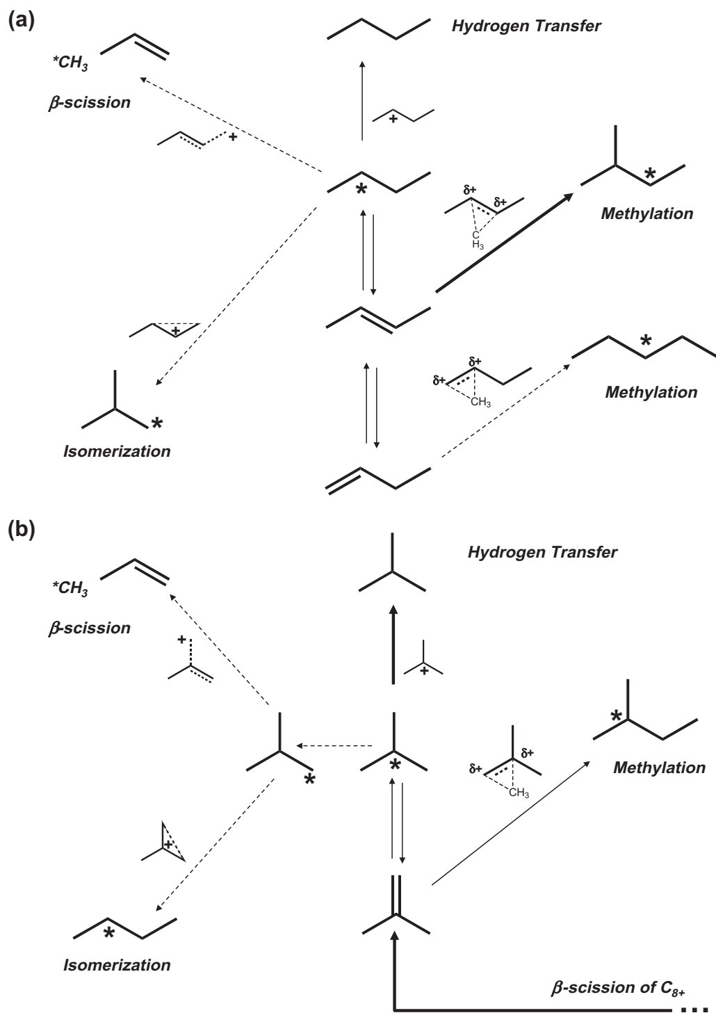
Scheme 4. Reaction pathways for (a) n -butyl species ( n -butenes and sec -butoxide) and (b) isobutyl species (isobutene and tert -butoxide) in acid-catalyzed dimethyl ether homologation pathways. Methylation of n -butene to isopentyl species occurs faster than hydrogen transfer to sec -butoxide. Methylation of isobutene to isopentyl species occurs slower than hydrogen transfer to tert -butoxide. Isomerization and \beta -scission of both sec -butoxide and tert -butoxide occur much more slowly than hydrogen transfer to these alkoxides and methylation of their alkenes.
