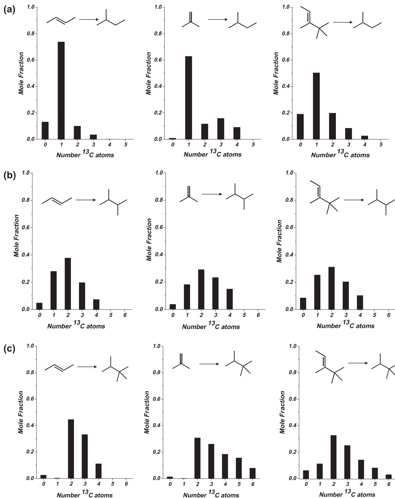
Fig. 7. Isotopologue distributions of (a) isopentane, (b) 2,3-dimethylbutane, and (c) triptane molecules produced from reactions between ^{13}\text{C} -labeled dimethyl ether (78 kPa) and 0.5 kPa unlabeled trans-2-butene (left), isobutene (middle), or 3,4,4-trimethyl-2-pentene (right) at 473 K on H-BEA (Si/Al = 12.5). We use the 85 amu fragment of triptane as a surrogate for the parent ion, because the former appears in much higher concentrations in the mass spectrometer than the latter. Reactions conducted at 473 K and space velocity of 0.025 \text{ mol inlet gas} [\text{mol Al s}]^{-1} with >90\% alkene conversion and less than 5% total carbon conversion (DME and alkene).
